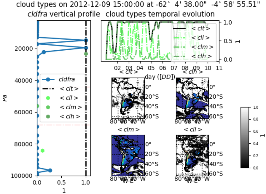
Figure 1: Vertical distribution of cloud fraction and the different cloud types at a given point (top left): cloud fraction ( cldfra , full circles with line in blue), mean total cloud fraction ( cldtmean , vertical dashed line), mean low-level cloud fraction ( cldlmean p \geq 680 hPa, dark green hexagon), mean mid-level ( cldmmean 680 < p \leq 440 hPa, green hexagon), mean high-level ( cldhmean p < 440 hPa, clear green hexagon). Temporal evolution of cloud types at the given point (top right). Map of cldtmean with colored topography beneath to show-up cloud extent (middle middle), map of cldhmean (middle right), map of cldmmean (bottom middle) and map of cldlmean (bottom right)
