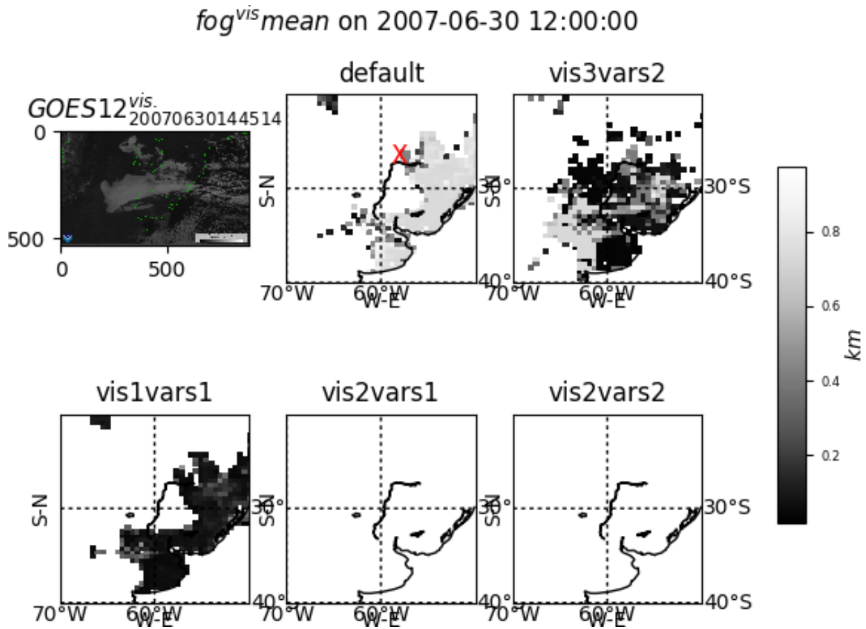
Figure 13: Comparison of the different configurations of the diagnostics of the mean fog visibility (in 1 hour) to the satellite image from GOES-12 at the same time in the visible channel (courtesy of NOAA-CLASS), default (fogvisibility=3, fogvars=1; top middle), vis3vars2 (top right), vis1vars1 (bottom left), vis2vars1 (bottom middle) and vis2vars2 (bottom right)
