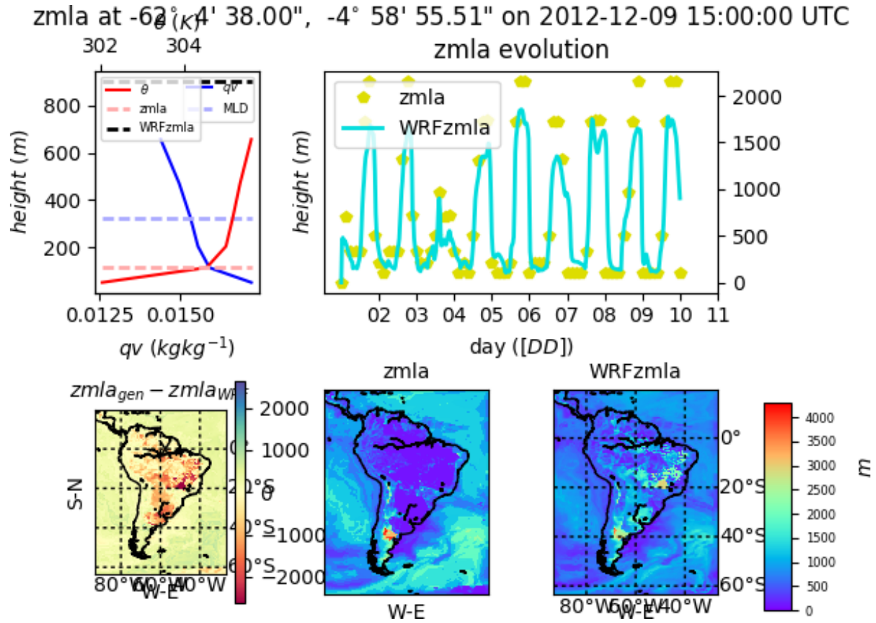
Figure 14: Vertical characteristics of the atmosphere at a given point (top left): potential temperature vertical profile ( \theta K, red line), vertical profile of mixing ratio ( qv kgkg^{-1} , blue line), mixed layer depth ( MLD , dashed horizontal line at 323.522 m), derived boundary layer height ( zmla , horizontal dashed line at 107.122 m and WRF derived pbl scheme value ( WRF_{zmla} at 903.017 m). Comparison of temporal evolutions (top right) between derived zmla (yellow stars) and WRF's pbl scheme (blue line). Map of differences between derived and WRF simulated ( zmla - zmla_{WRF} , bottom left), zmla map (bottom middle) and zmla_{WRF} (bottom right)
